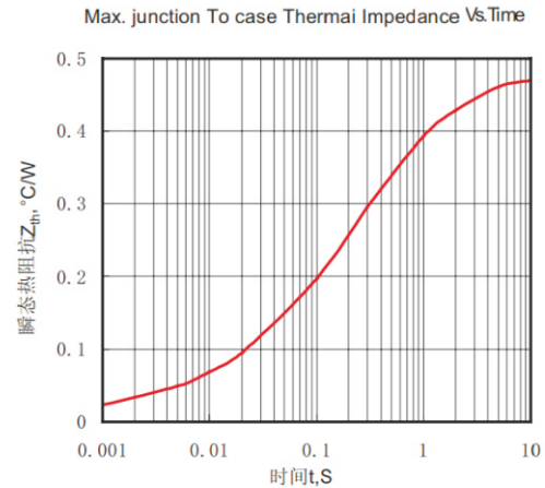
Fig.2 瞬态热阻抗抗曲线
